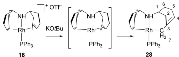
Scheme 8. Allyl complex 28 from 16 . Numbers given in complex 28 are the labeling key for its NMR spectroscopic data.
