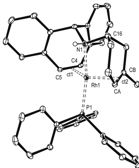
Figure 4. ORTEP plot (at 30% ellipsoid probability) of structure 16 . The noncoordinated anion, two thf molecules and carbon-bonded hydrogen atoms are omitted for clarity. Selected bond lengths [Å] and angles [°] (ct1 = centroid C4=C5, ct2 = centroid CA=CB): Rh1–N1 2.1199(22), Rh1–P1 2.2815(7), Rh1–ct1 2.045(3), Rh1–ct2 2.128(3), Rh1–C4 2.151(3), Rh1–C5 2.177(3), Rh1–CA 2.230(3), Rh–CB 2.2450(3), C4=C5 1.418(4), CA=CB 1.385(4); N1–Rh1–P1 168.79(7), ct1–Rh1–ct2 143.59(11).
