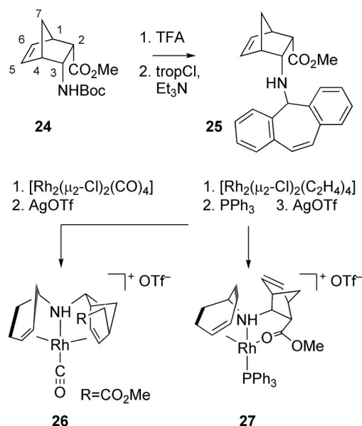
Scheme 7. Synthesis of ligand 25 from 24 and complexes 26 , 27 . Numbers given in ligand 24 are the labeling key for the NMR spectroscopic data of compounds 24 – 27 .
