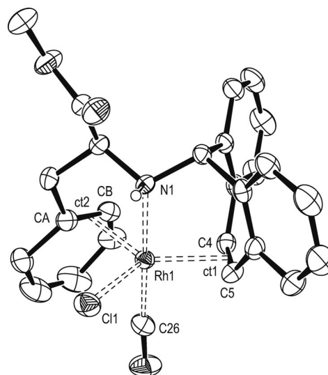
Figure 1. ORTEP plot (at 30% ellipsoid probability) of structure 5 . Carbon-bound hydrogen atoms and one solvent molecule are omitted for clarity. Selected bond lengths [Å] and angles [°] (ct1 = centroid C4=C5, ct2 = centroid CA=CB): Rh1–N1 2.151(3), Rh1–C26 1.867(4), Rh1–Cl 2.526(3), Rh1–ct1 2.074(4), Rh1–ct2 2.193(5), Rh1–C4 2.176(5), Rh1–C5 2.212(5), Rh1–CA 2.321(5), Rh1–CB 2.282(5), C4=C5 1.430(6), CA=CB 1.396(7); N1–Rh1–C26 174.28(12), ct1–Rh1–ct2 129.18(18).
