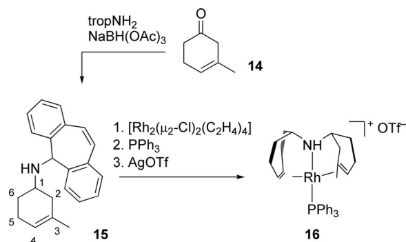
Scheme 5. Synthesis of ligand 15 and complex 16 . Numbers given in ligand 15 are the labeling key for the NMR spectroscopic data of compounds 15 and 16 .
