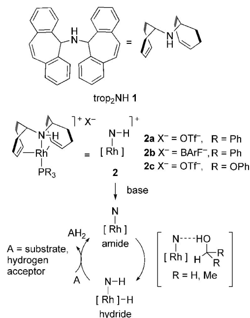
Scheme 1. Trop 2 NH (1), [Rh(trop 2 NH)(PPh 3 )]OTf (2) and proposed catalytic cycle. The benzo groups of the trop units in the ligand are omitted for clarity and only denoted by bold lines in this and all subsequent schemes. OTf - = trifluoromethanesulfonate anion, BArF - = tetrakis[3,5-bis(trifluoromethyl)phenyl]borate anion.
