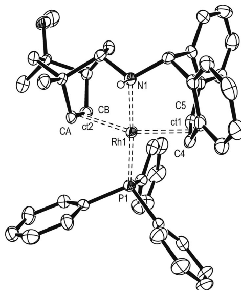
Figure 5. ORTEP plot (at 30% ellipsoid probability) of structure 23 . Carbon-bonded hydrogen atoms and the disordered triflate anion are omitted for clarity. Selected bond lengths [Å] and angles [°] (ct1 = centroid C4=C5, ct2 = centroid CA=CB): Rh1–N1 2.114(4), Rh1–P1 2.2762(15), Rh1–ct1 2.073(5), Rh1–ct2 2.153(5), Rh1–C4 2.168(5), Rh1–C5 2.215(5), Rh1–CA 2.203(4), Rh–CB 2.320(6), C4=C5 1.418(8), CA=CB 1.393(7); N1–Rh1–P1 176.58(12), ct1–Rh1–ct2 153.22(21).
