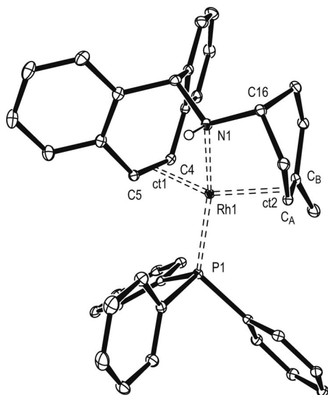
Figure 3. ORTEP plot (at 30% ellipsoid probability) of structure 13 . The noncoordinated anion and carbon-bonded hydrogen atoms are omitted for clarity. Selected bond lengths [Å] and angles [°] (ct1 = centroid C4=C5, ct2 = centroid CA=CB): Rh1–N1 2.1069(15), Rh1–P1 2.2772(4), Rh1–ct1 2.026(2), Rh1–ct2 2.165(2), Rh1–C4 2.1277(17), Rh1–C5 2.1663(17), Rh1–CA 2.2129(17), Rh–CB 2.3317(18), C4=C5 1.420(3), CA=CB 1.383(3); N1–Rh1–P1 162.84(5), ct1–Rh1–ct2 143.98(7).
