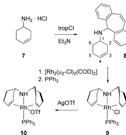
Scheme 3. Synthesis of ligand 8 and complexes 9, 10. Numbers given in ligand 8 are the labelling key for the NMR spectroscopic data of compounds 8–10.
