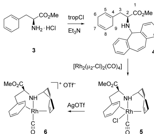
Scheme 2. Synthesis of 4 and the rhodium complexes 5, 6. Numbers given in ligand 4 are the labeling key for the NMR spectroscopic data of compounds 3–6.
