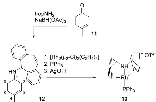
Scheme 4. Synthesis of ligand 12 and complex 13 . Numbers given in ligand 12 are the labeling key for the NMR spectroscopic data of compounds 12 and 13 .
