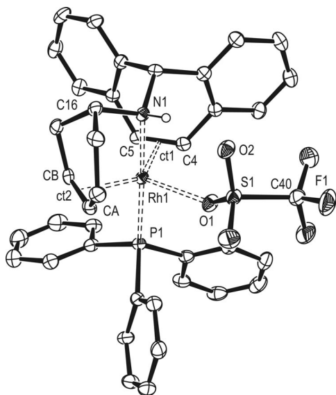
Figure 2. ORTEP plot (at 30% ellipsoid probability) of structure 10 . Carbon-bonded hydrogen atoms are omitted for clarity. Selected bond lengths [Å] and angles [°] (ct1 = centroid C4=C5, ct2 = centroid CA=CB): Rh1–N1 2.135(3), Rh1–P1 2.075(4), Rh1–O1 2.347(3), Rh1–ct1 2.053(4), Rh1–ct2 2.075(4), Rh1–C4 2.182(4), Rh1–C5 2.161(4), Rh1–CA 2.210(4), Rh–CB 2.168(4), C4=C5 1.418(6), CA=CB 1.395(6), N1–O2 3.094(8); N1–Rh1–P1 177.62(9), ct1–Rh1–ct2 135.05(14).
