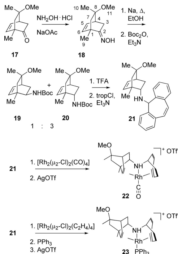
Scheme 6. Synthesis of ligand 21 and complexes 22 , 23 . Numbers given in ligand 18 are the labeling key for the NMR spectroscopic data of compounds 17 – 23 .
